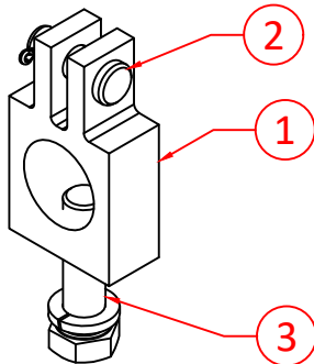
MACHINED STYLE WITH LINER ACCESS (STYLE 2)
